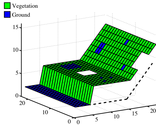
Figure 6.6: Simulated sensor data, showing transition from ground to tall vegetation with missing and ambiguous data. The dashed line gives the true ground height
