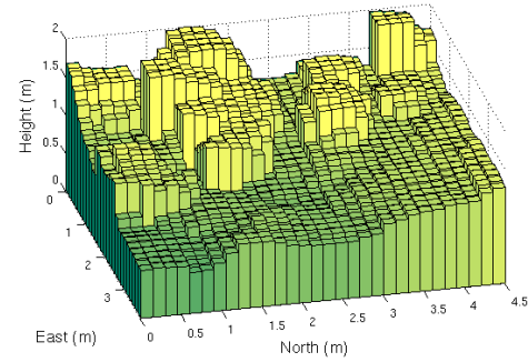
Figure 4.25: Highest point surface
