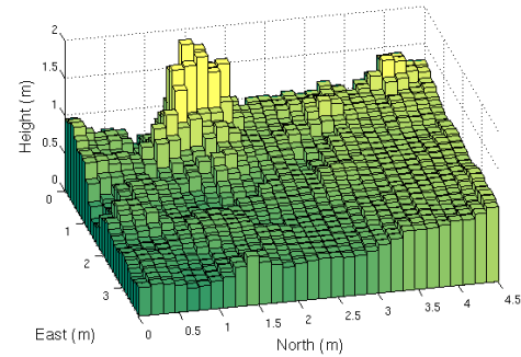
Figure 4.27: Learned result removes the vegetation but keeps the person
