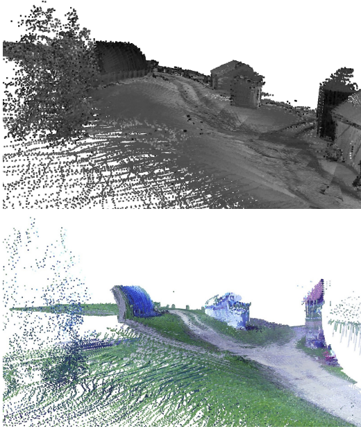
Figure 1.2: Map of farm test site buildings using both ladars as the vehicle drove on a path to the field. The top figure shows laser reflectance, and the bottom figure shows the colorized points (the color camera has a narrower field of view than the laser).
