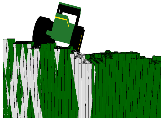
Figure 6.27: Lowest hit or pass-through and independent classification (the diagonal pattern in the classifications is a rendering artifact)
