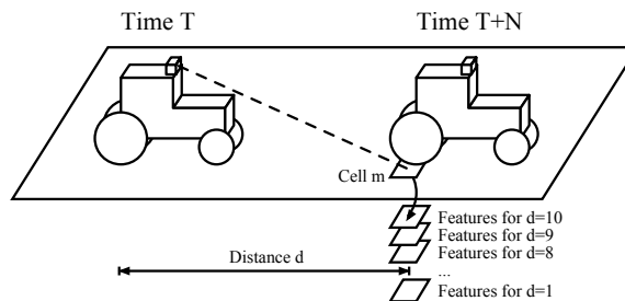
Figure 4.3: Approach for training traversable terrain
