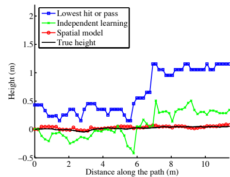
Figure 7.9: Height prediction comparison for right wheel
