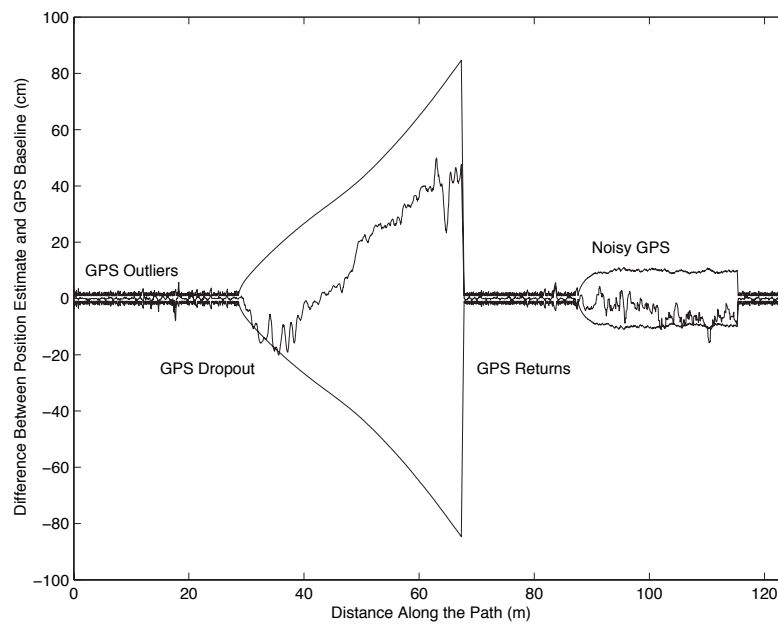
Figure A.3: Position error and uncertainty from figure A.2
